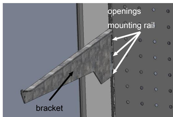
Fig. 9: Hang up bracket (without/with LED-bar)
